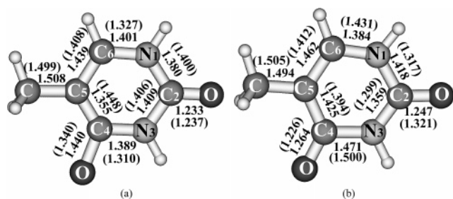
Figure 2. Equilibrium geometries of the lowest {}^1n\pi^* (a) and {}^1\pi\pi^* (b) excited states of thymine, determined at the CC2/cc-pVDZ level with C_s symmetry constraint. Bond lengths are given in angstroms. The bond lengths determined at the CASSCF/cc-pVDZ level are given in parentheses.
