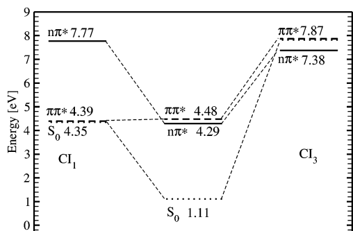
Figure 5. Energy-level diagram of the S_0 (dotted line), the {}^1n\pi^* (solid line), and the {}^1\pi\pi^* (dashed line) states of thymine, calculated with the CASPT2 method at the equilibrium geometry of the {}^1n\pi^* excited state and the CI_1 and CI_3 conical intersections. The energies (relative to the minimum energy of the ground state) are given in electronvolts.
