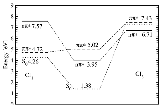
Figure 6. Energy-level diagram of the S_0 (dotted line), the {}^1n\pi^* (solid line), and the {}^1\pi\pi^* (dashed line) states of thymine, calculated with the CC2 method at the equilibrium geometry of the {}^1n\pi^* excited state and the CI_1 and CI_3 conical intersections. The energies (relative to the minimum energy of the ground state) are given in electronvolts.
